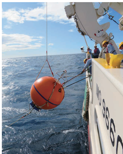
係留流速計の回収作業 Recovery of a mooring of current meter
