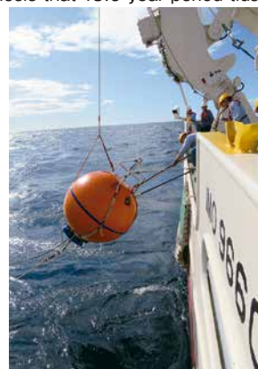
係留流速計の回収作業 Recovery of a mooring of current meter
